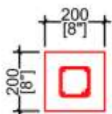
(C1) COLUMN DETAIL (C1) 200X200 CONCRETE BEAM 4T10 R6@150 C/C
