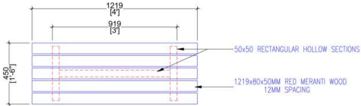
PLAN
